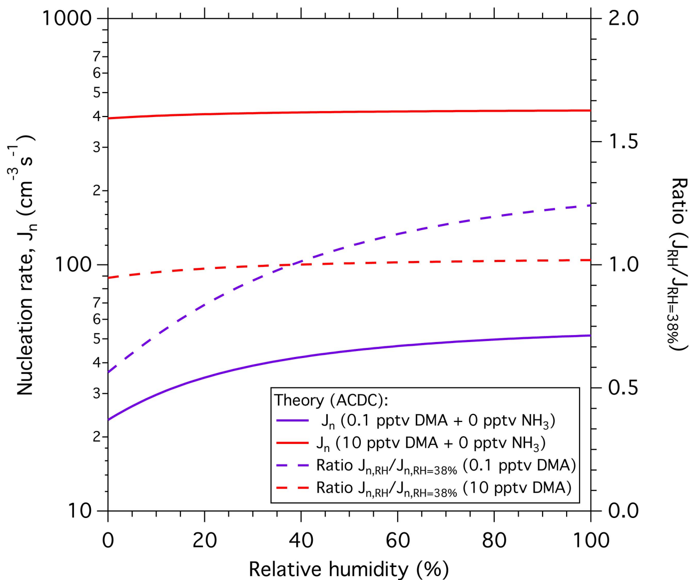
Extended Data Figure 2 | Theoretical dependence of amine ternary nucleation rates on RH. Modelled neutral nucleation rates as a function of RH (left-hand scale) at 2.0 \times 10^6 \text{ cm}^{-3} [ \text{H}_2\text{SO}_4 ] and 278 K, and either 0.1 p.p.t.v.
